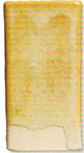
CO-6 Supernova over V-308 Yellow
